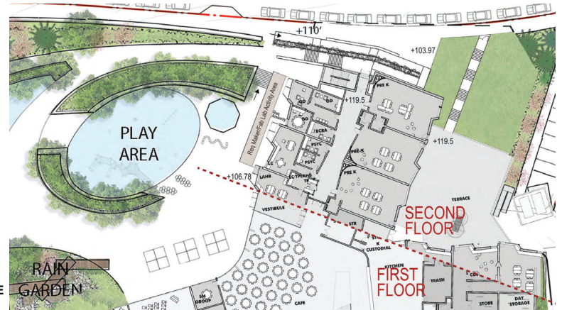
NORTH ENTRANCE OPTION A
