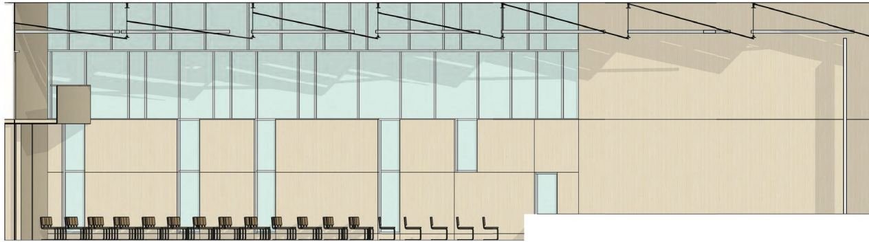
MULTI-PURPOSE ROOM, FACADE INTERIOR ELEVATION
